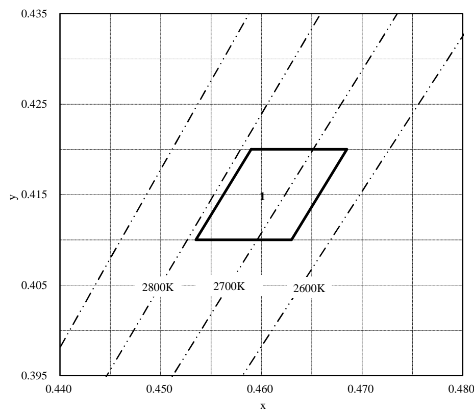
Chromaticity Diagram
